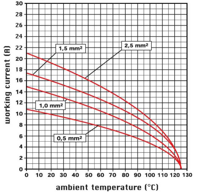
diagram CSH 16 poles
